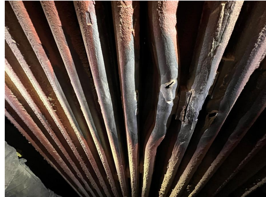
Reheat Tubes Inside Boiler
